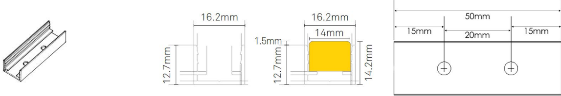
CONT V SLIM NJ AL PROFILE 1M (1m aluminum profile)
